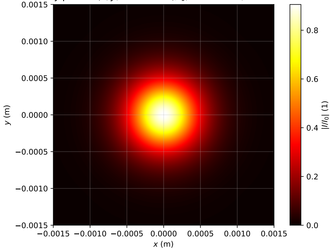
Intensity profile I(x, y, z = 3.821m)/I_0 , P_{in}=0.8P_{cr} , artificial time
